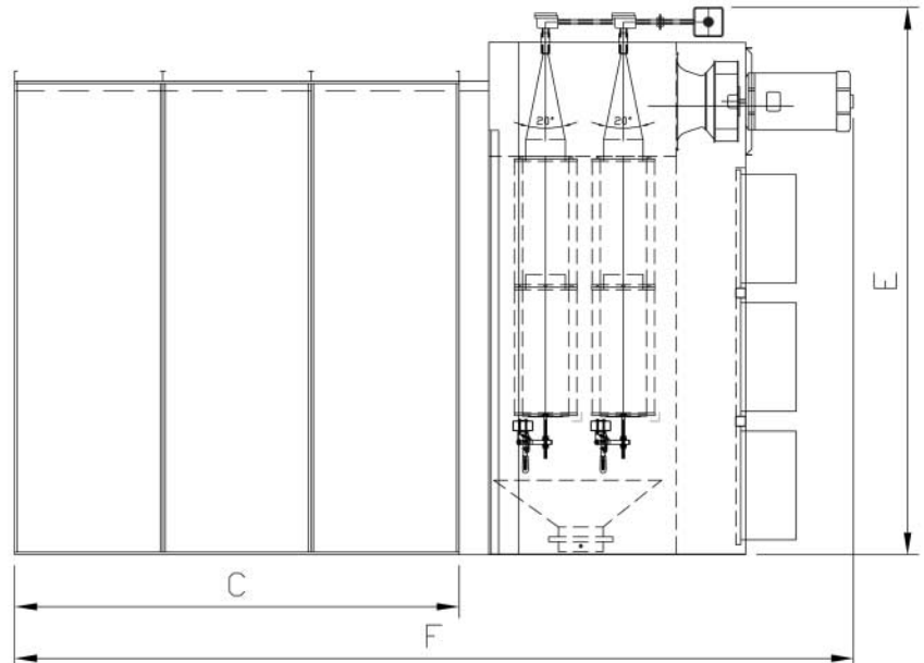
SIDE ELEVATION VIEW SHOWN WITH OPTIONAL FLUIDIZING HOPPER
